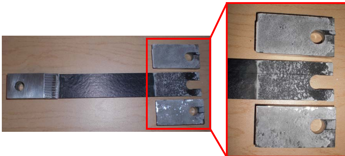
Failure mode observed in composite tests
