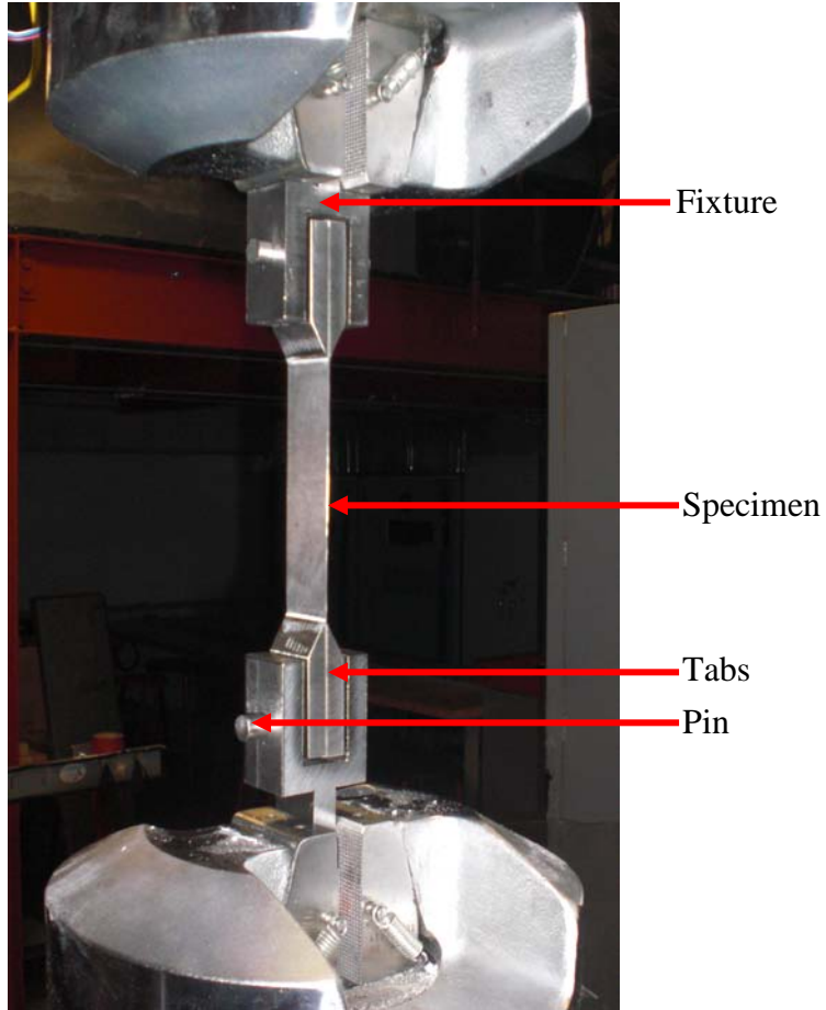
Experimental arrangement for composite tensile testing
